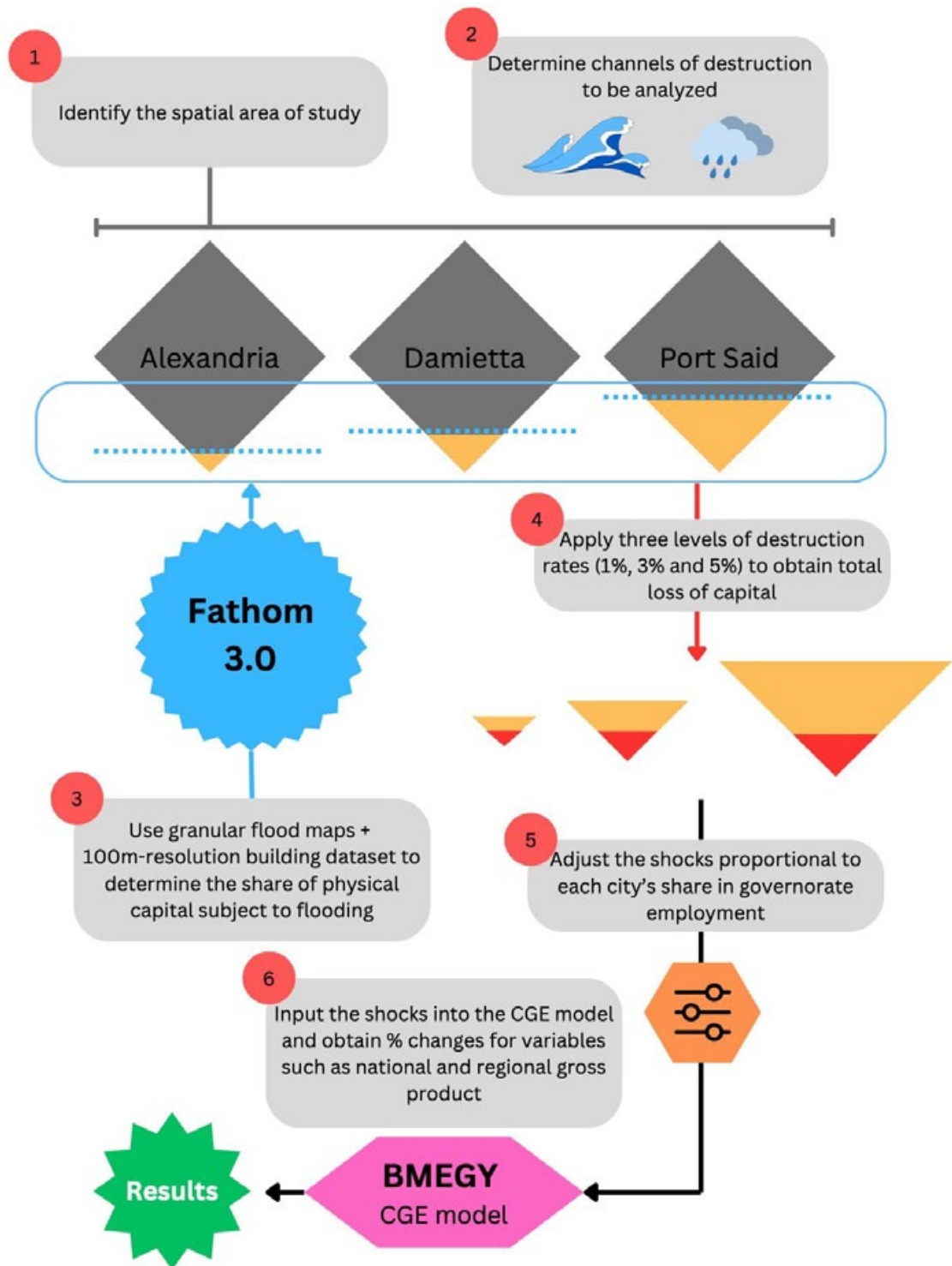
Figure 3 Methodology Flowchart
